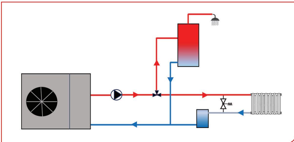
Figure 2: Zone control (e.g. zone valves) – Auto Bypass + Volumiser
